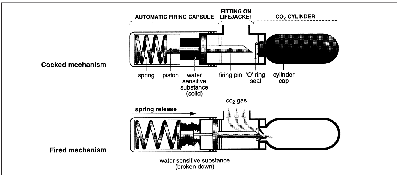
Automatic inflation mechanism
